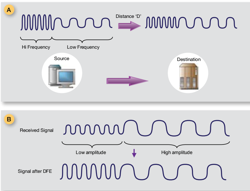
Figure 2: 6 Gb/s SAS-2 overcomes attenuation effects by de-emphasizing lower frequency components at the transmitter (see Figure 2A) as well as by selectively boosting higher frequency components on the receive side (see Figure 2B) using an equalization method called Decision Feedback Equalization (DFE). Developers designing or troubleshooting SATA Gen-3 equipment must resolve attenuation and jitter issues differently as SATA Gen-3 does not support either de-emphasis or equalization.
